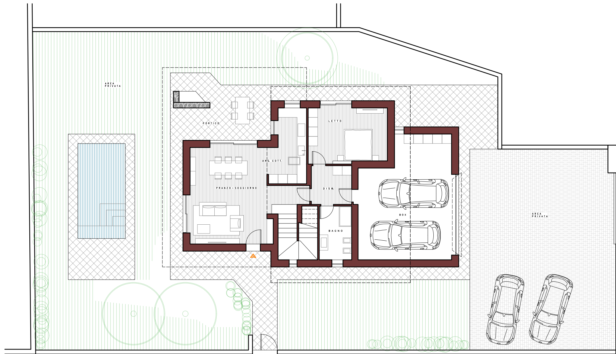
VILLA "C" PIANO TERRA
